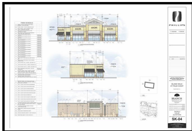
Shops D Color Elevations
